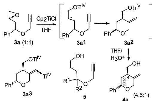
Scheme 2. Radical cyclization of epoxides.
