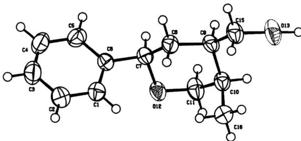
Figure 4. X-ray picture of 7a 2 .
