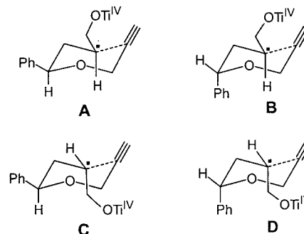
Figure 2. Transition complexes of the intermediate radical.
